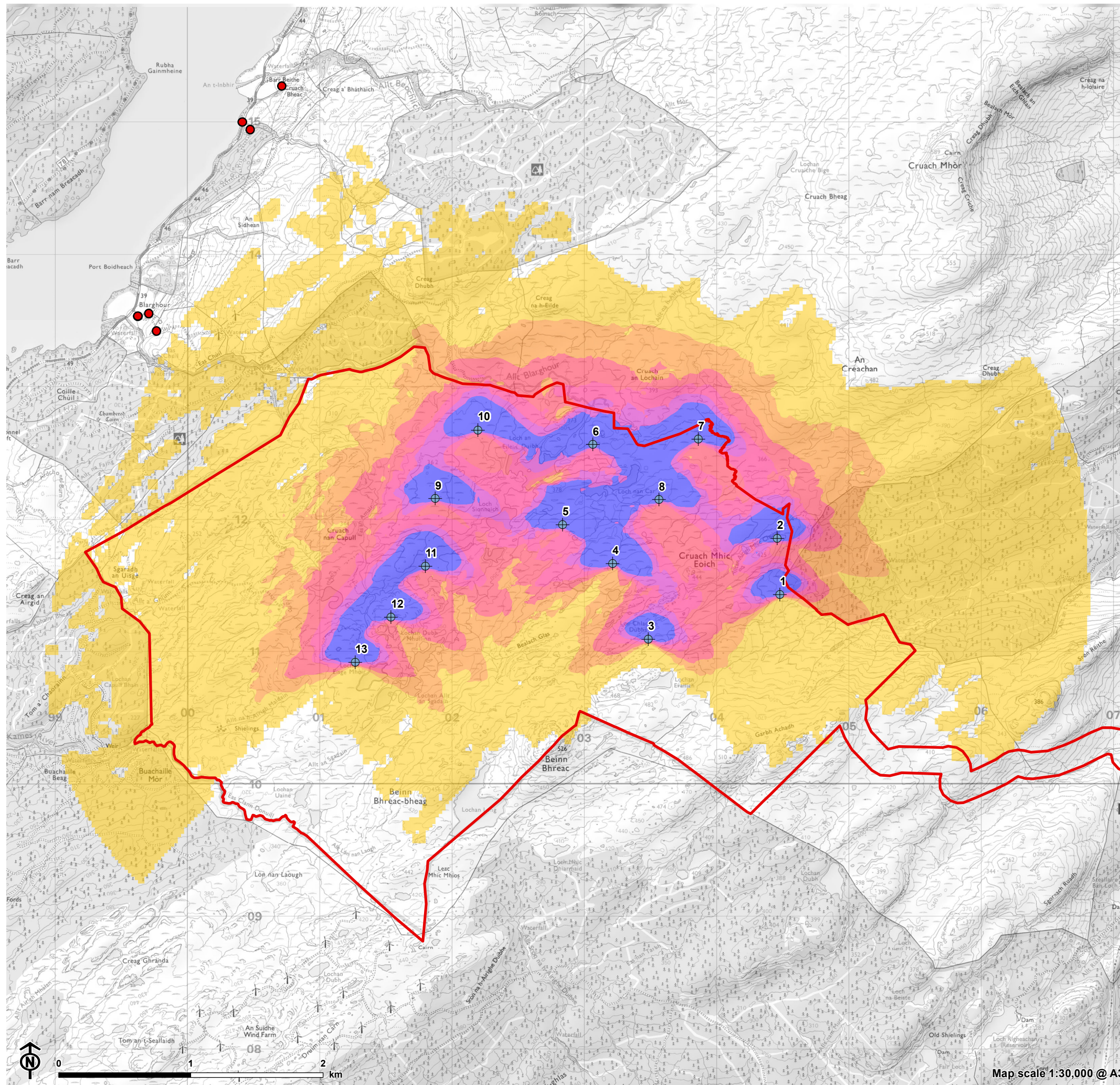
Figure 2.1: Maximum Theoretical Shadow Flicker
