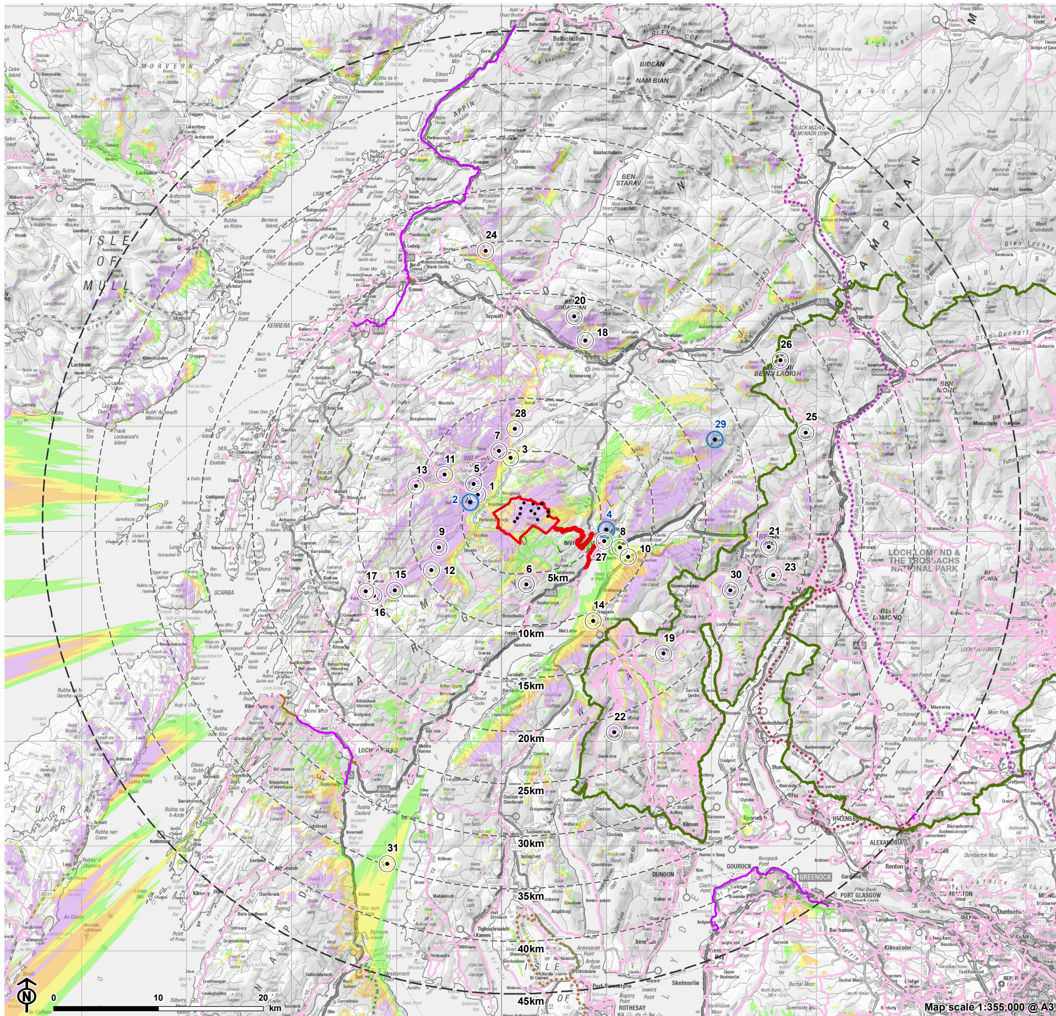
Figure 6.1.2a: Blade Tip Height (180m) Zone of Theoretical Visibility (ZTV) and Viewpoint Locations
