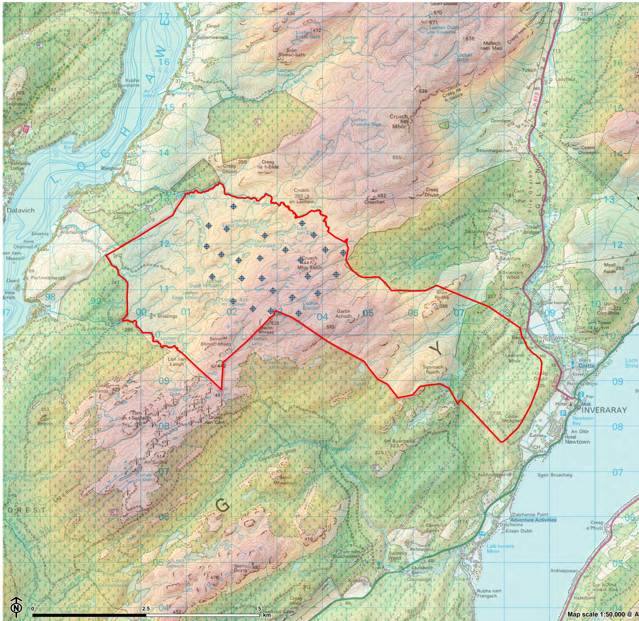
Figure 3.1: Proposed Turbine Layout
