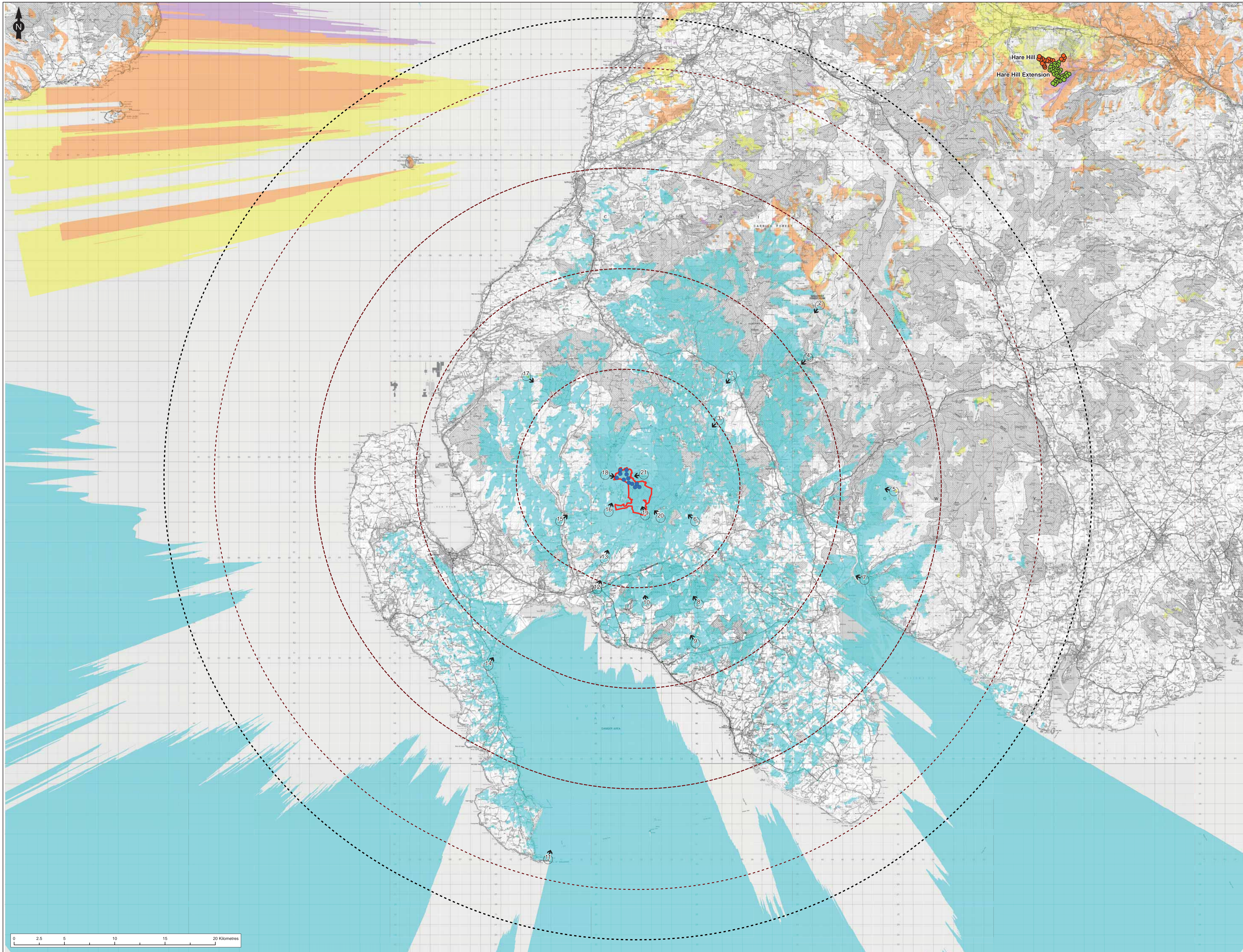
Figure Title Figure 5.7g: Cumulative ZTV Proposed development, Hare Hill and Hare Hill Extension
