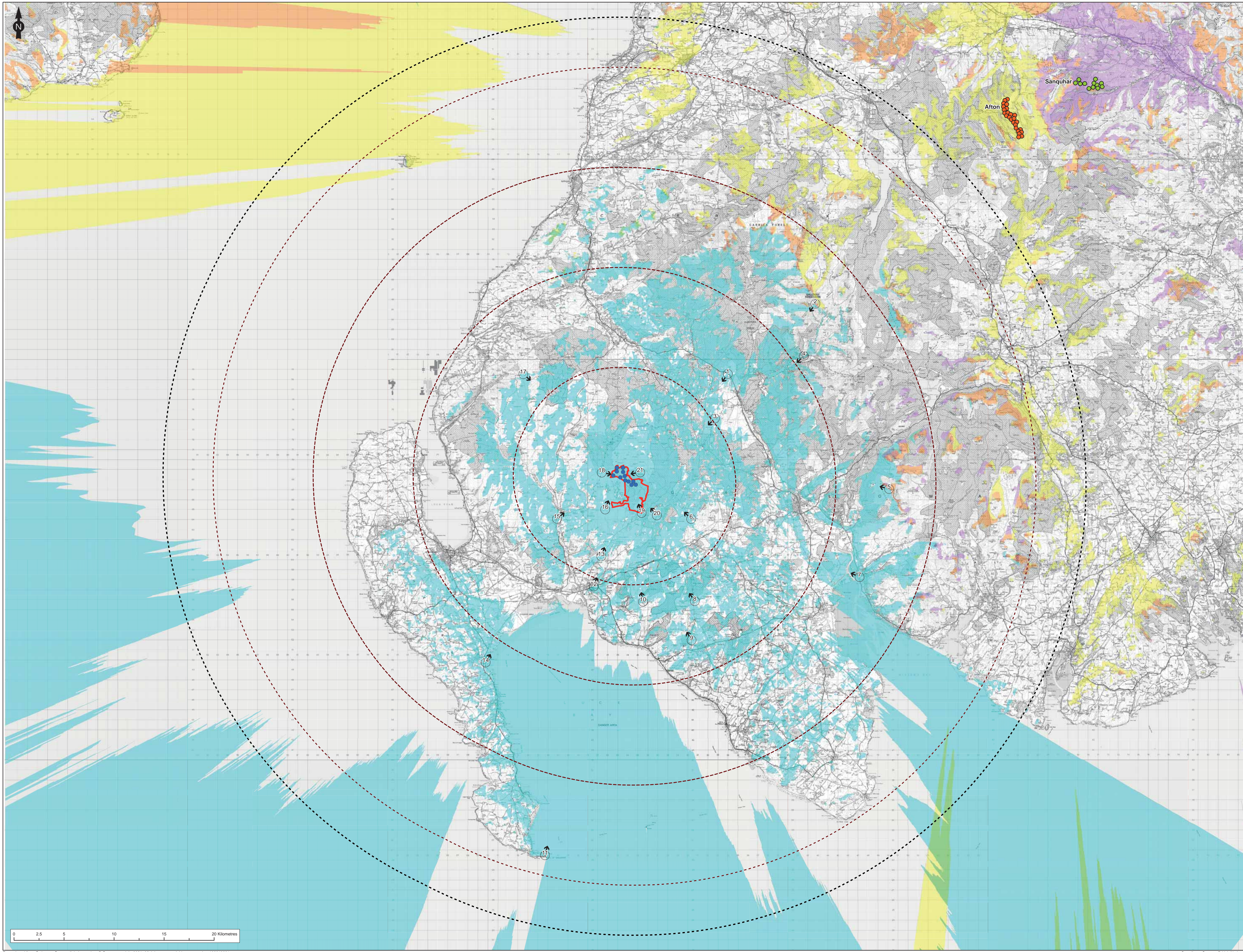
Figure Title Figure 5.7h: Cumulative ZTV Proposed development, Afton and Sanquhar
