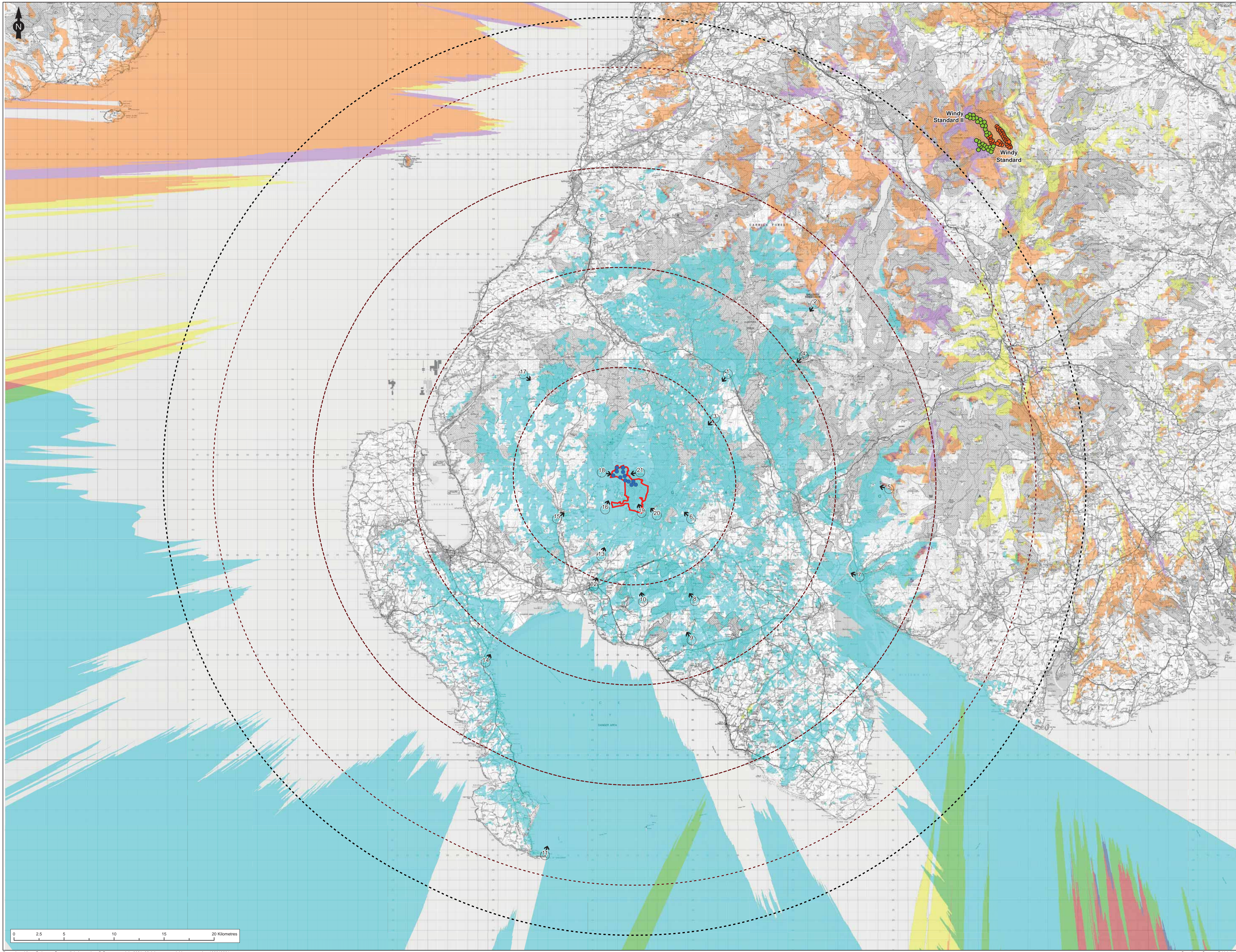
Figure Title Figure 5.7f: Cumulative ZTV Proposed development, Windy Standard and Windy Standard II
