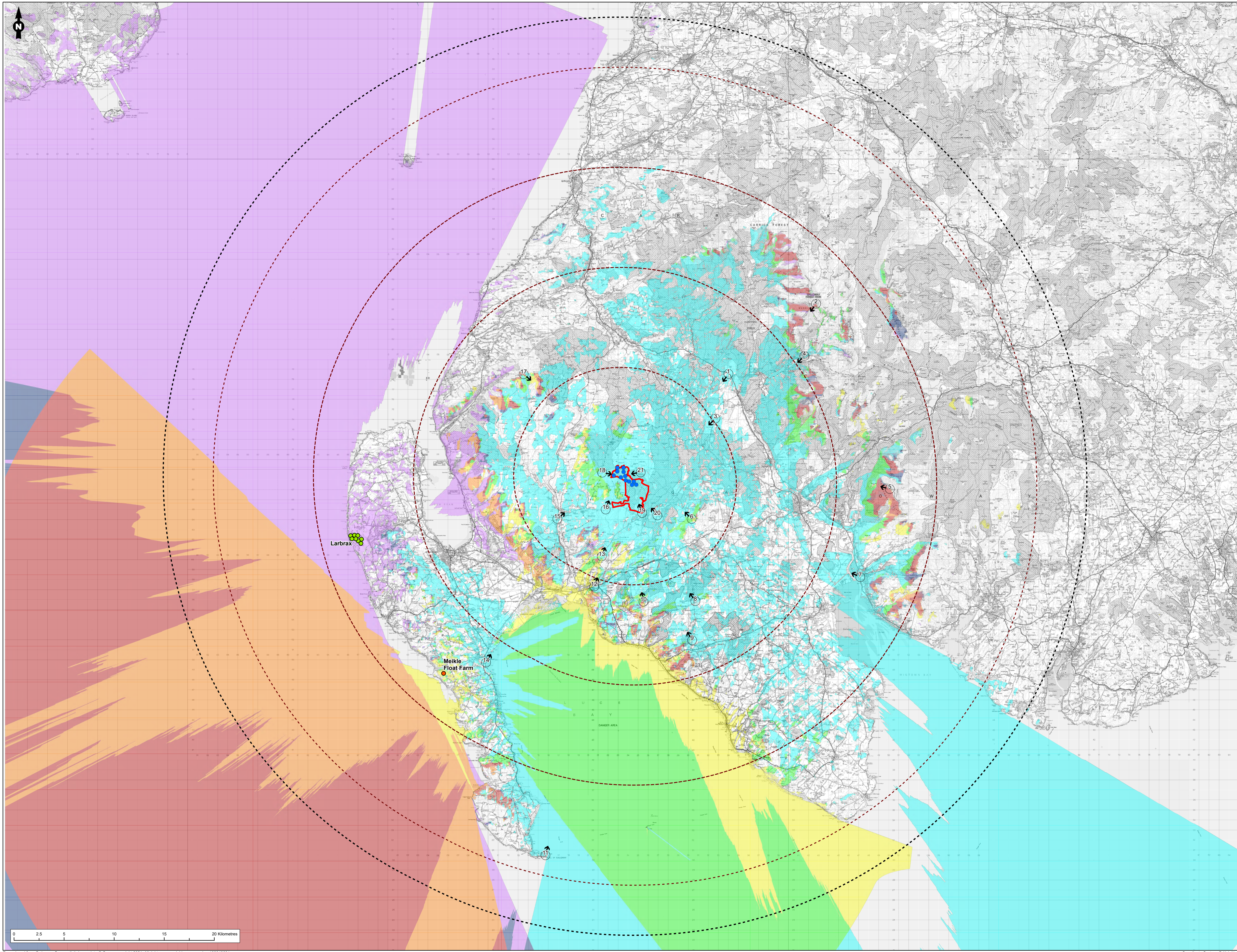
Figure Title Figure 5.7w: Cumulative ZTV Proposed development, Meikle Float Farm and Larbrax
