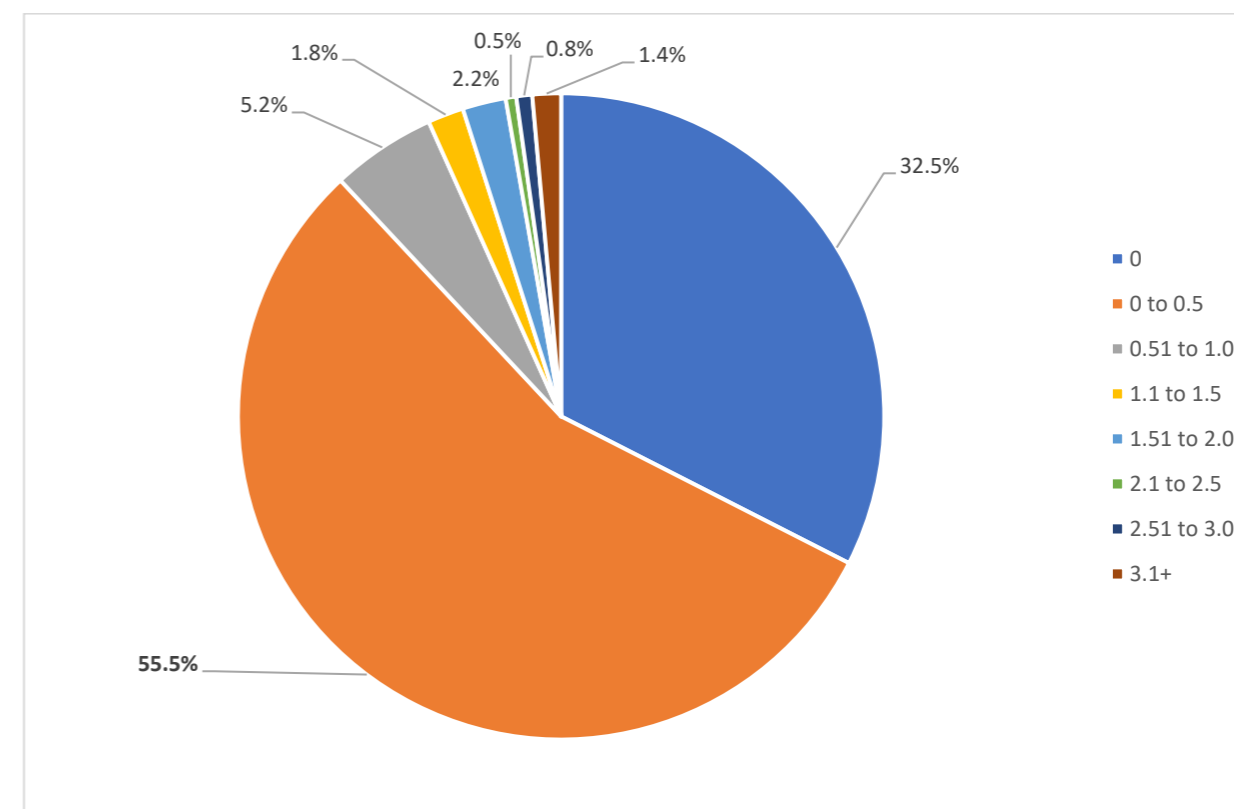
Graph 2.3.1: Percentage Peat Depth Categories (All Surveys Combined)
