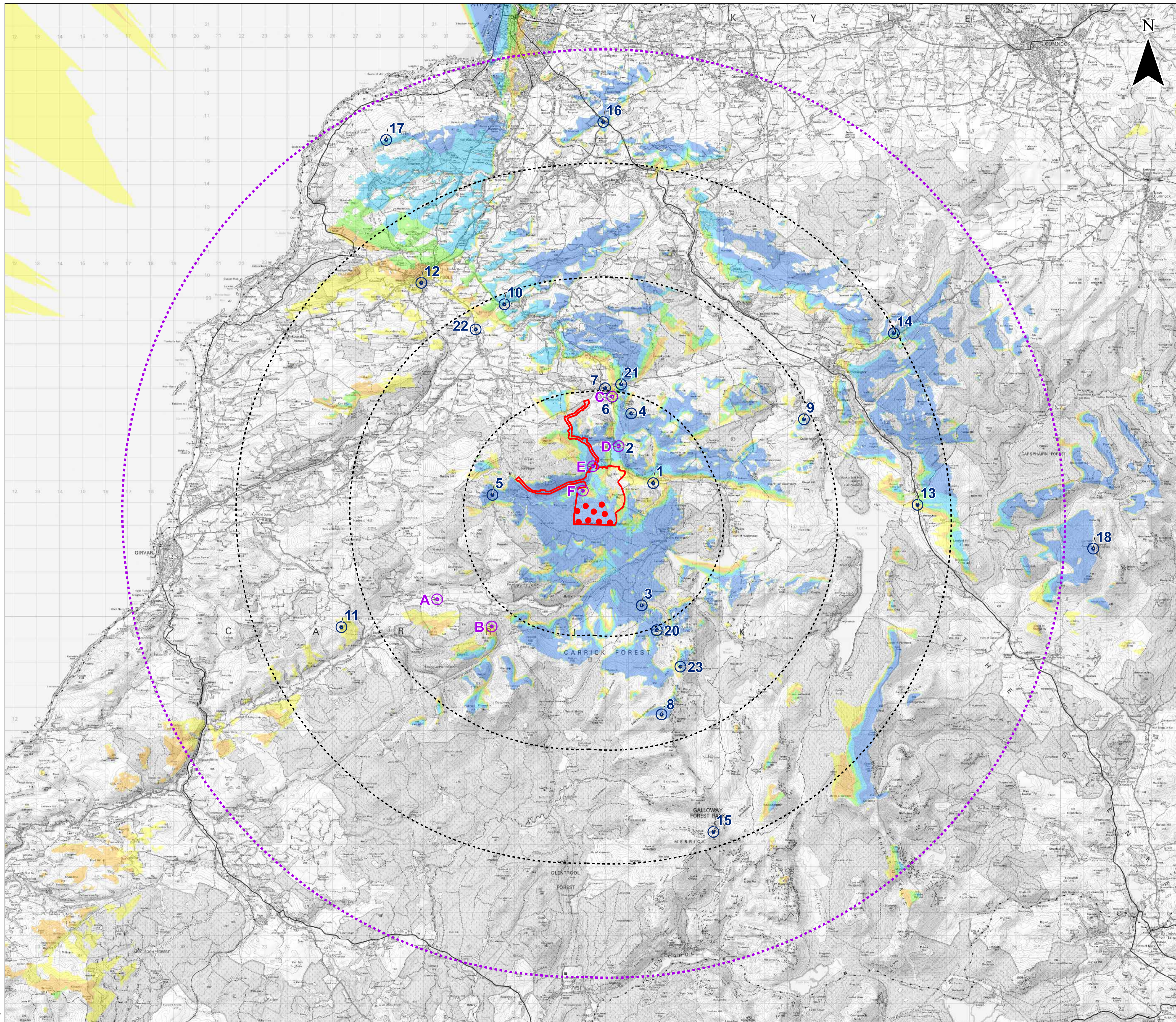
Hub Height ZTV with Viewpoints (20km)
