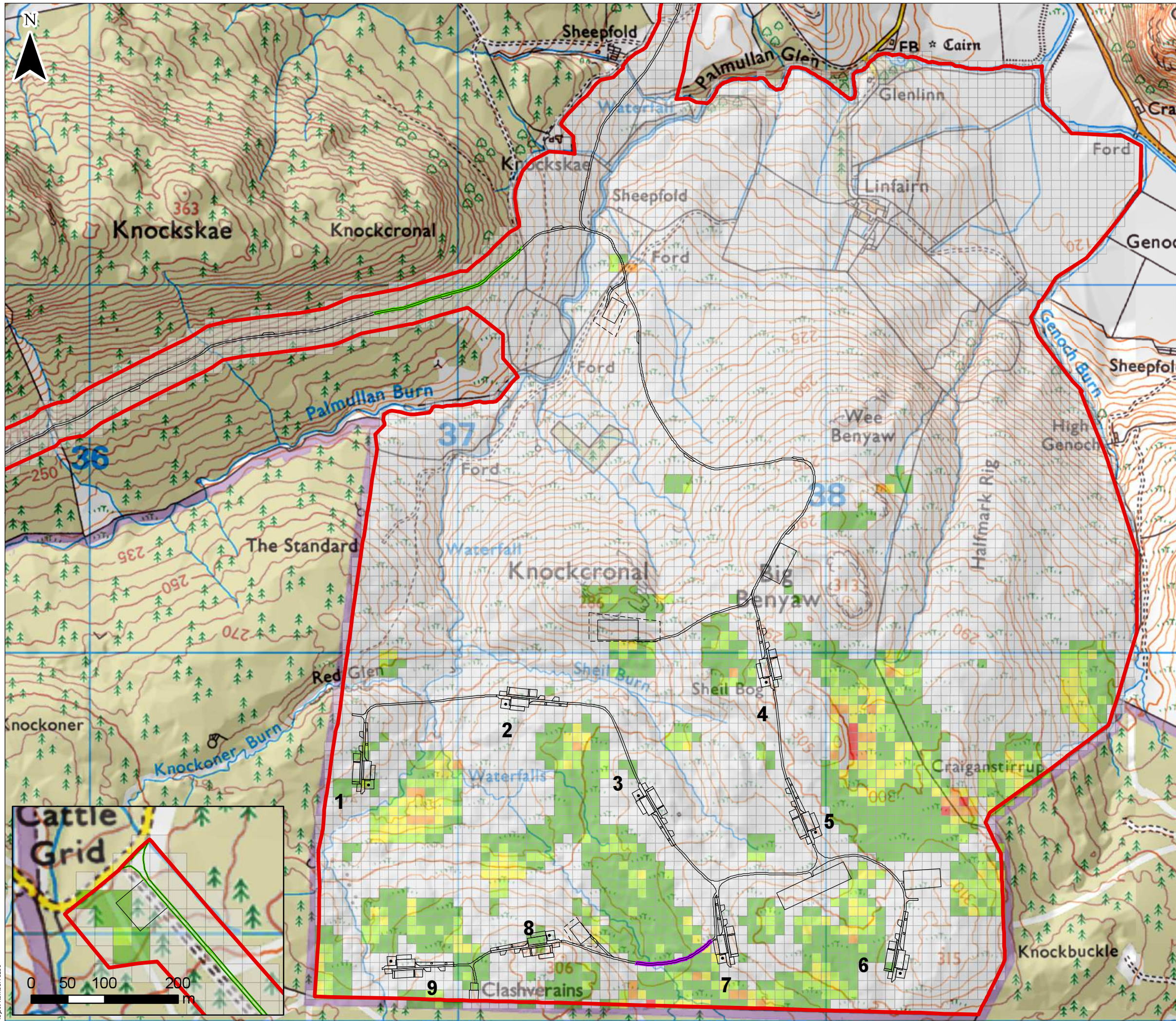
Figure 9.4.7 Factor of Safety (Lower Bound Estimate)
